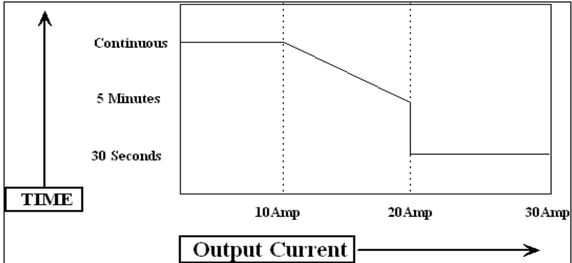
Graph 1* : Operating time on 30A range with current into a short circuit at 20°C Continuous current in available up to 10A output.
